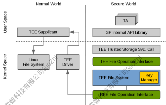
图 6-5: OP-TEE REE FS Secure Storage 软件架构
