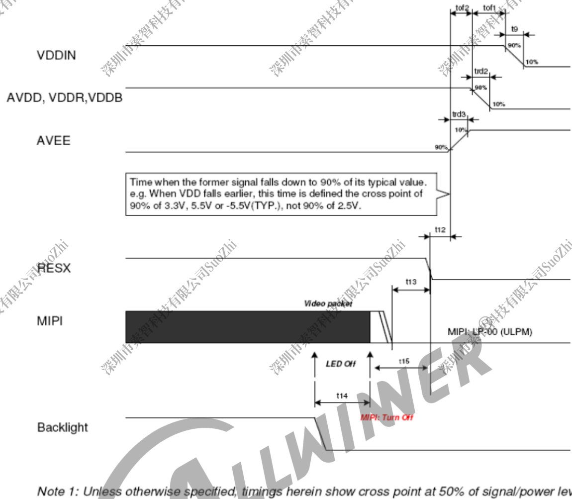
图 4-4: power off
